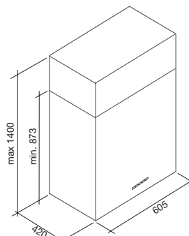
Altaire Top Isola / Island 60 600 m 3 /h
