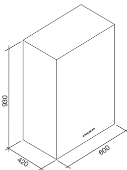
Altaire Top Parete / Wall 60 600 m 3 /h
